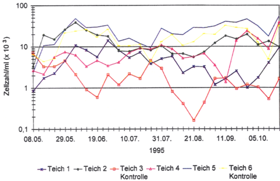
Abb. 2: Populationsdynamik Scenedesmus sp. (2-zelliges Zönobium)
