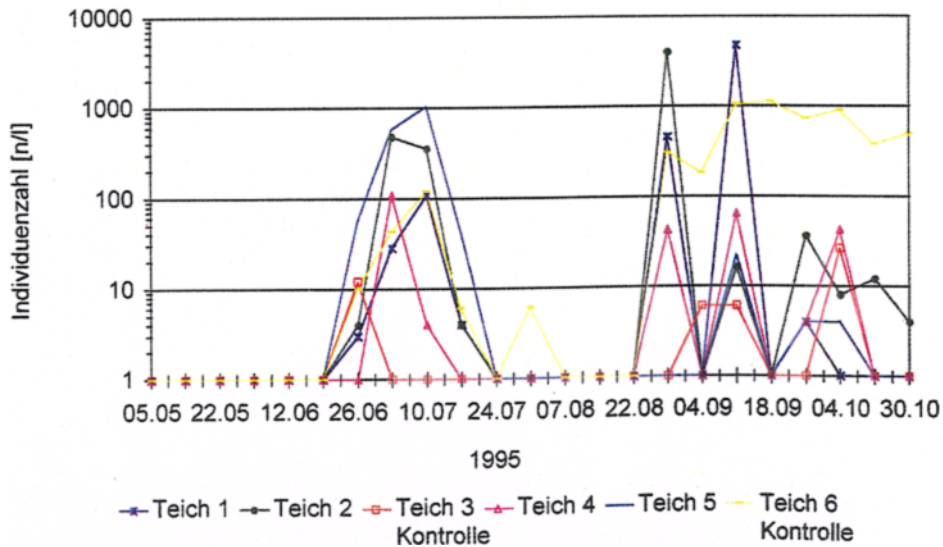
Abb. 3: Populationsdynamik Keratella quadrata
